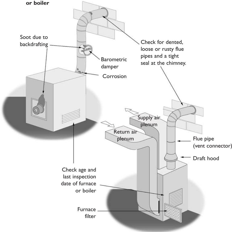
Conventional natural gas or propane forced air furnace
